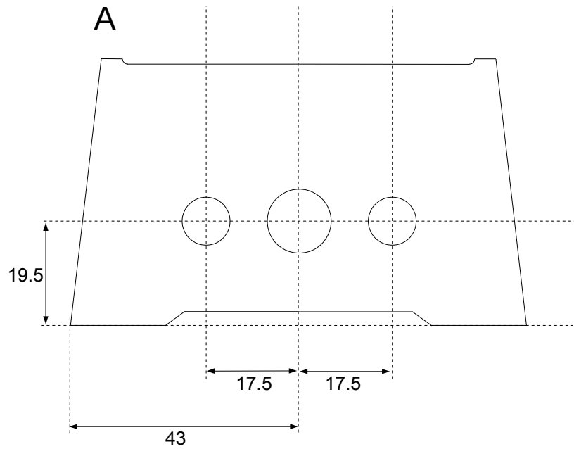
Drilling pattern recommended for PCB mounted jacks. This pattern suits the Rixen PCB template
