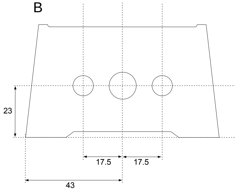
Drilling pattern recommended for off board jacks. This pattern is optimised for 16mm x 16mm body jacks to fit between two circuit boards
